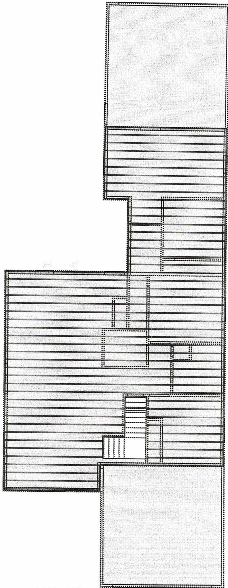
FLOOR JOIST FRAMING PLAN
