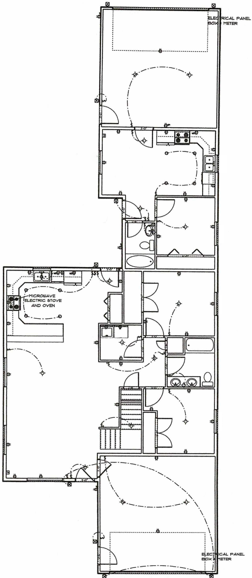
ELECTRICAL PLAN
