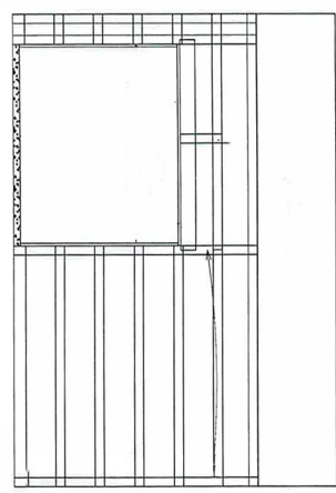
OVERHEAD DOOR OPTION SIDE ELEVATION
