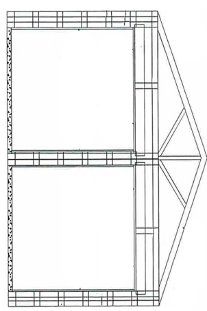
FRONT ELEVATION DOUBLE OVERHEAD DOOR
